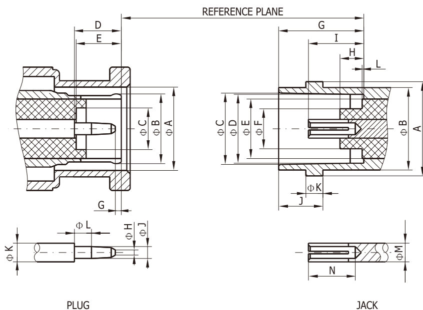
界面尺寸 (mm) Interface Dimensions in mm
